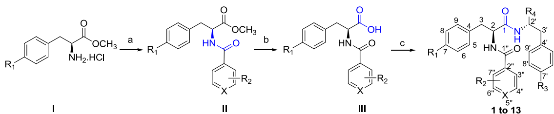
Scheme 1. Synthesis of compounds 4a–4n . Reagents and conditions: (a) substituted benzoic acid or isonicotinic acid, DCC, DMAP, \text{CH}_2\text{Cl}_2 , rt, 8 h; (b) 1.0 M NaOH, MeOH, rt; and (c) 4-substituted L-phenylalanine methyl ester hydrochloride or 4-substituted L-phenylalaninol, \text{CH}_2\text{Cl}_2 , IBCF, NMM, -5^\circ\text{C} .
