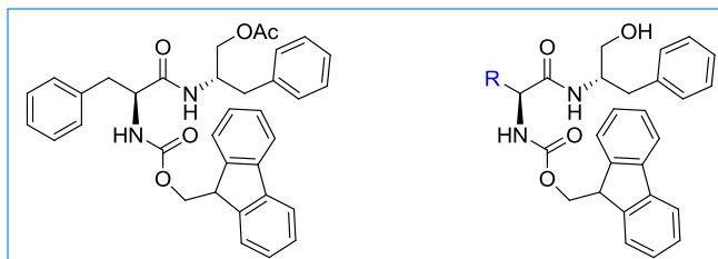
Fig. 2. Hsieh reported Fmoc-based dipeptides [13].
