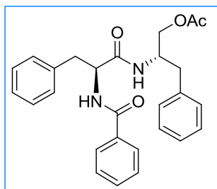
Fig. 1. The structure of MTS.
